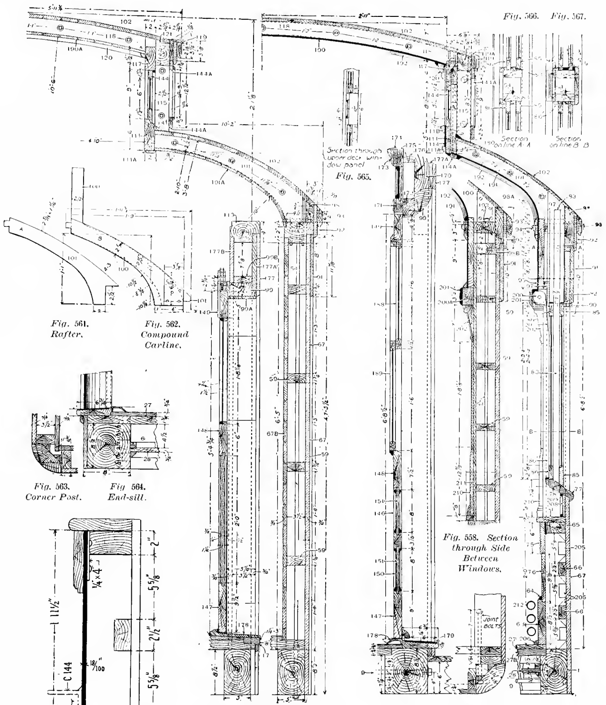
Cross Sections of Baggage Car. Cross Sections of Passenger Car.
